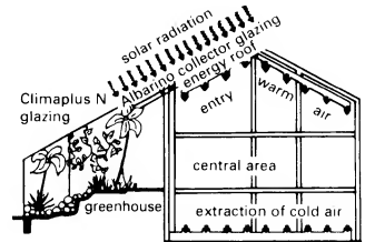
8 The function of hypocaustic gable wall heating
